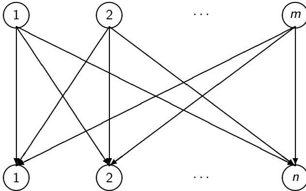
Figure: Bipartite Network Structure of Classical SPE Models
