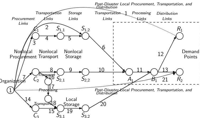
Figure: Disaster Relief Supply Chain Network Topology for Mexico Example and its Variant
